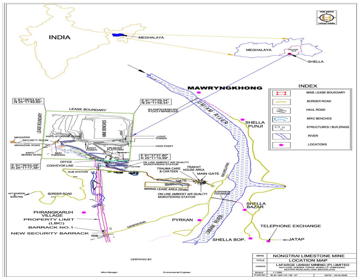
Figure 2.1: Location of Nongtraí Limestone Mine
