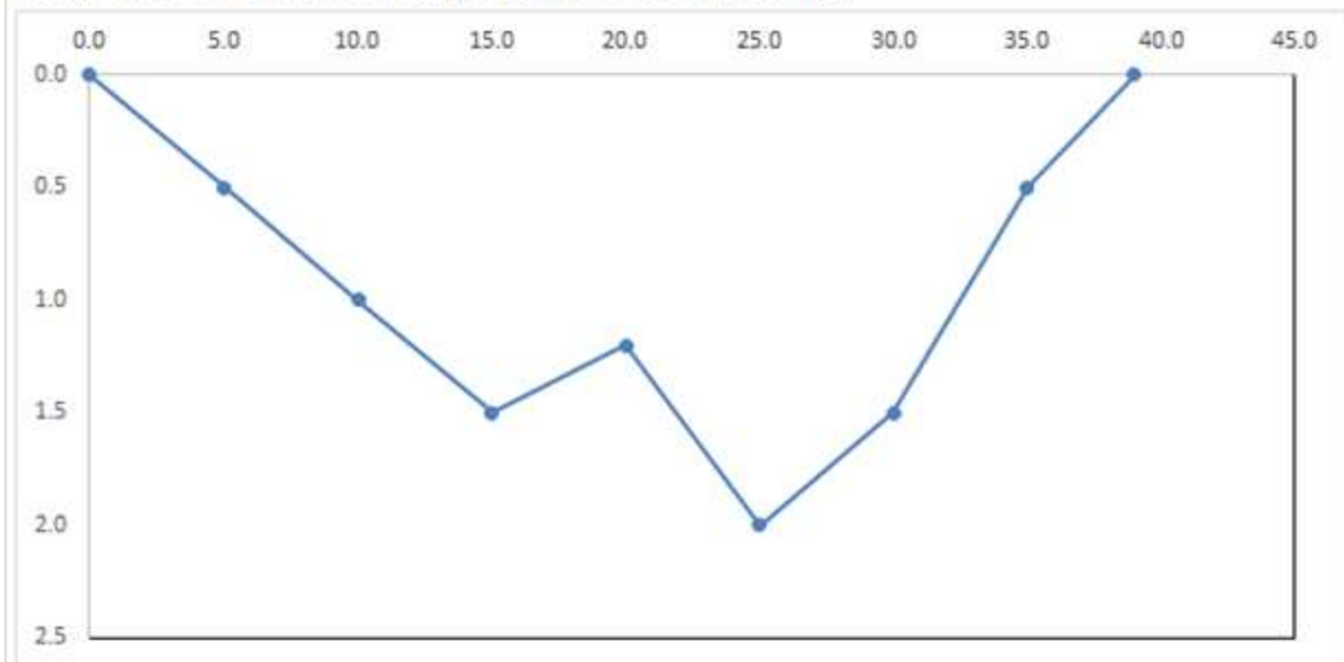
CROSS SECTION OF WATER FLOW MEASUREMENT AT DOWNSTREAM UMIAM RIVER TOP OF THE BRIDGE (DURING FAIR WEATHER)
